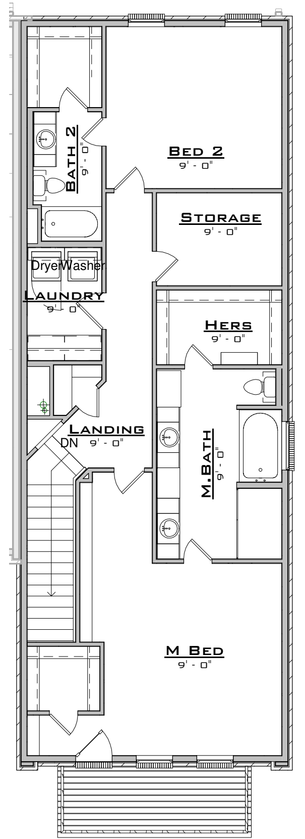
2 SECOND 1/8" = 1'-0"
