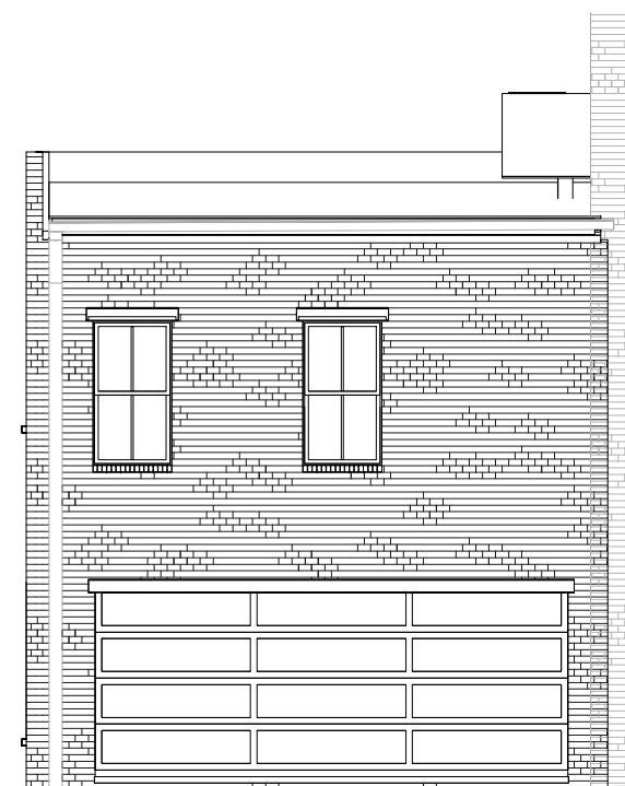
5 REARS 1/8" = 1'-0"
