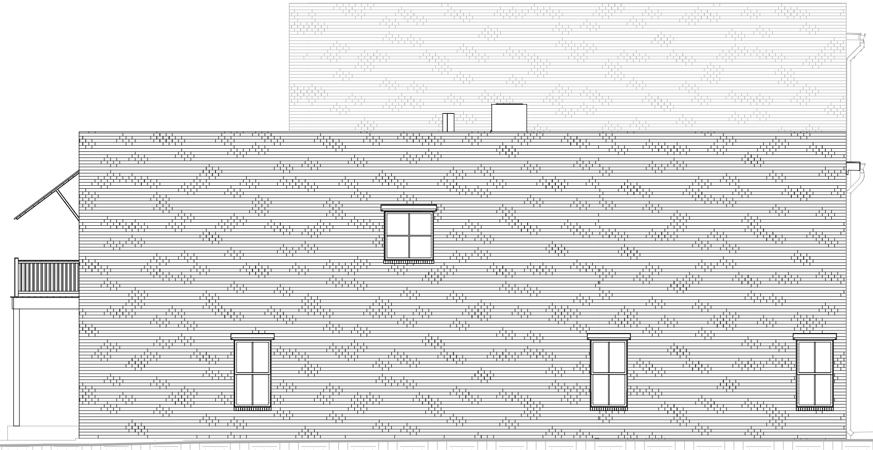
3 RIGHTS 1/8" = 1'-0"
