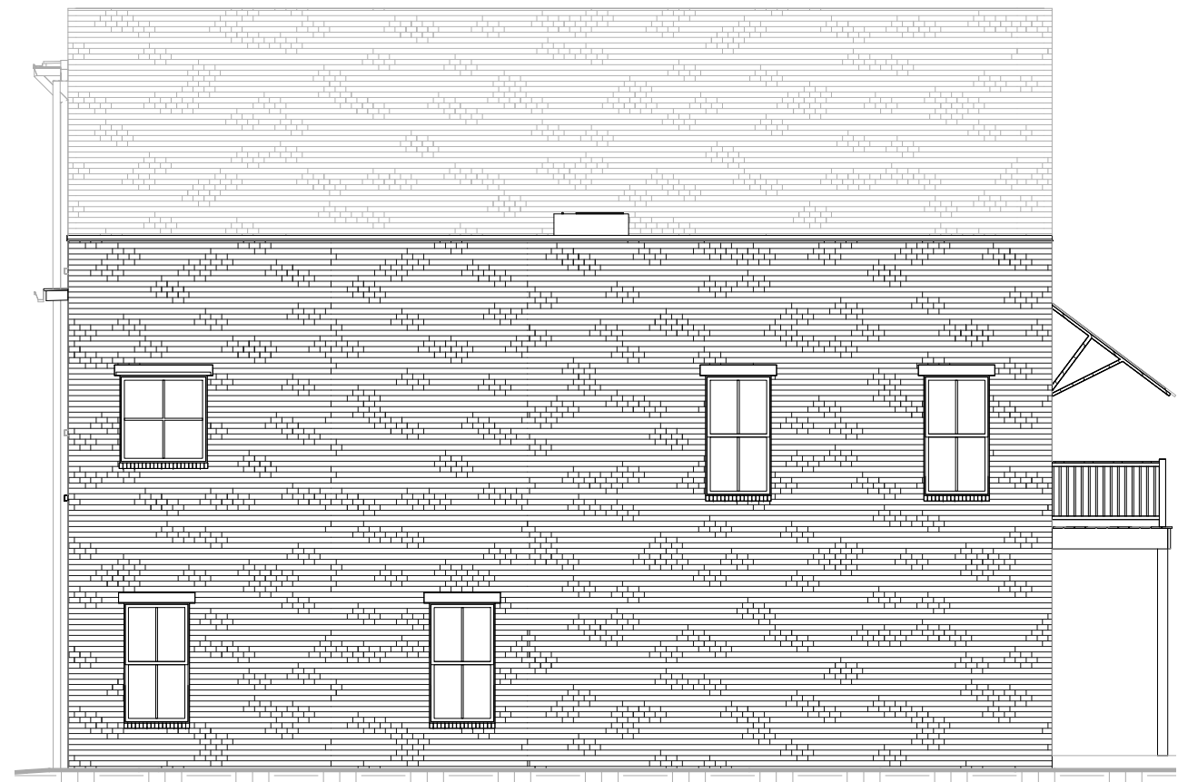
5 LEFTS 1/8" = 1'-0"
