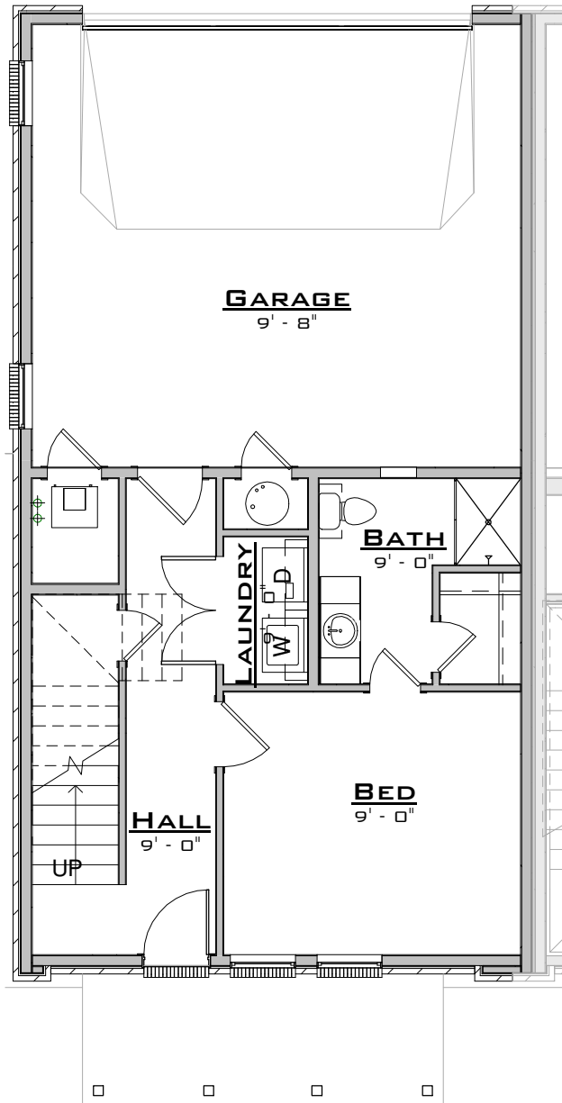
1 FIRST 1/8" = 1'-0"
