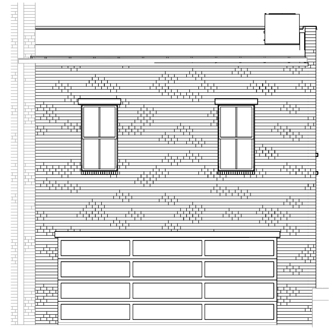
4 REARS 1/8" = 1'-0"
